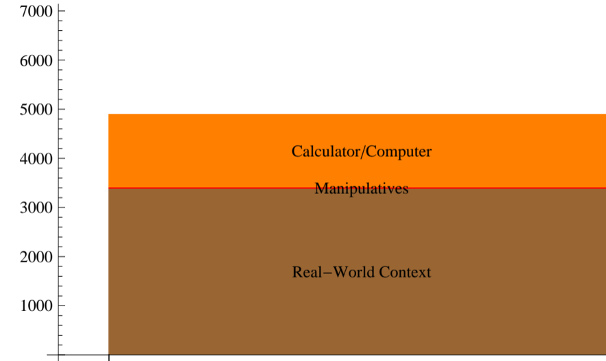
CPMP Total
