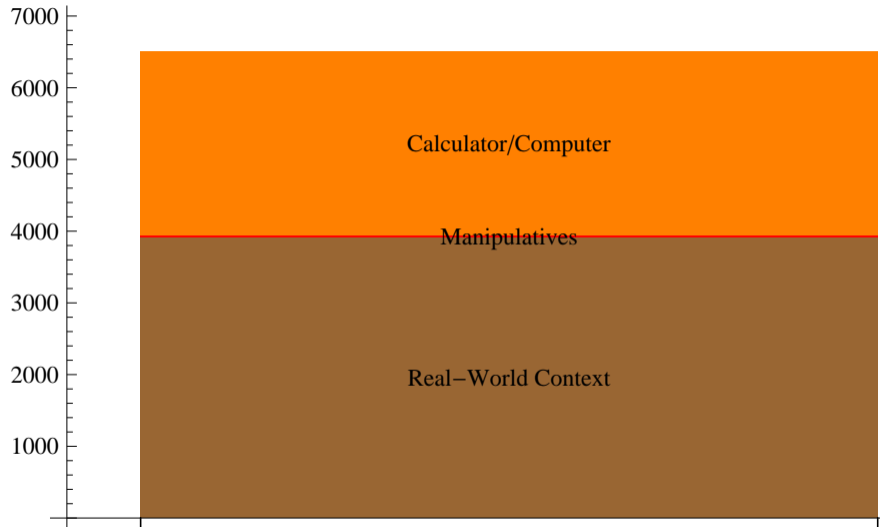
UCSMP Total
